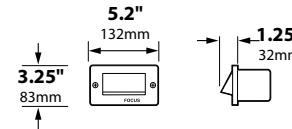
SL-30: Mounting Holes on all models 4-1/2" on center
